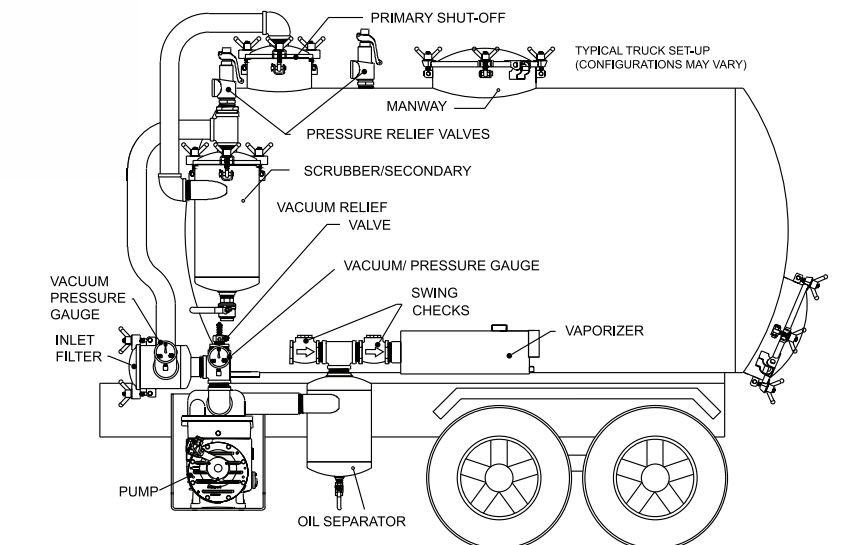
Typical Truck Set-Up (Configurations May Vary)
